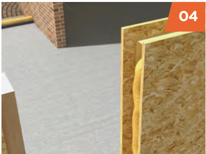
04 Expanding urethane sealant is used between all panel joints for superior airtightness.
